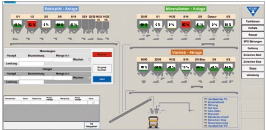
PCS35 screen with silo fill levels
